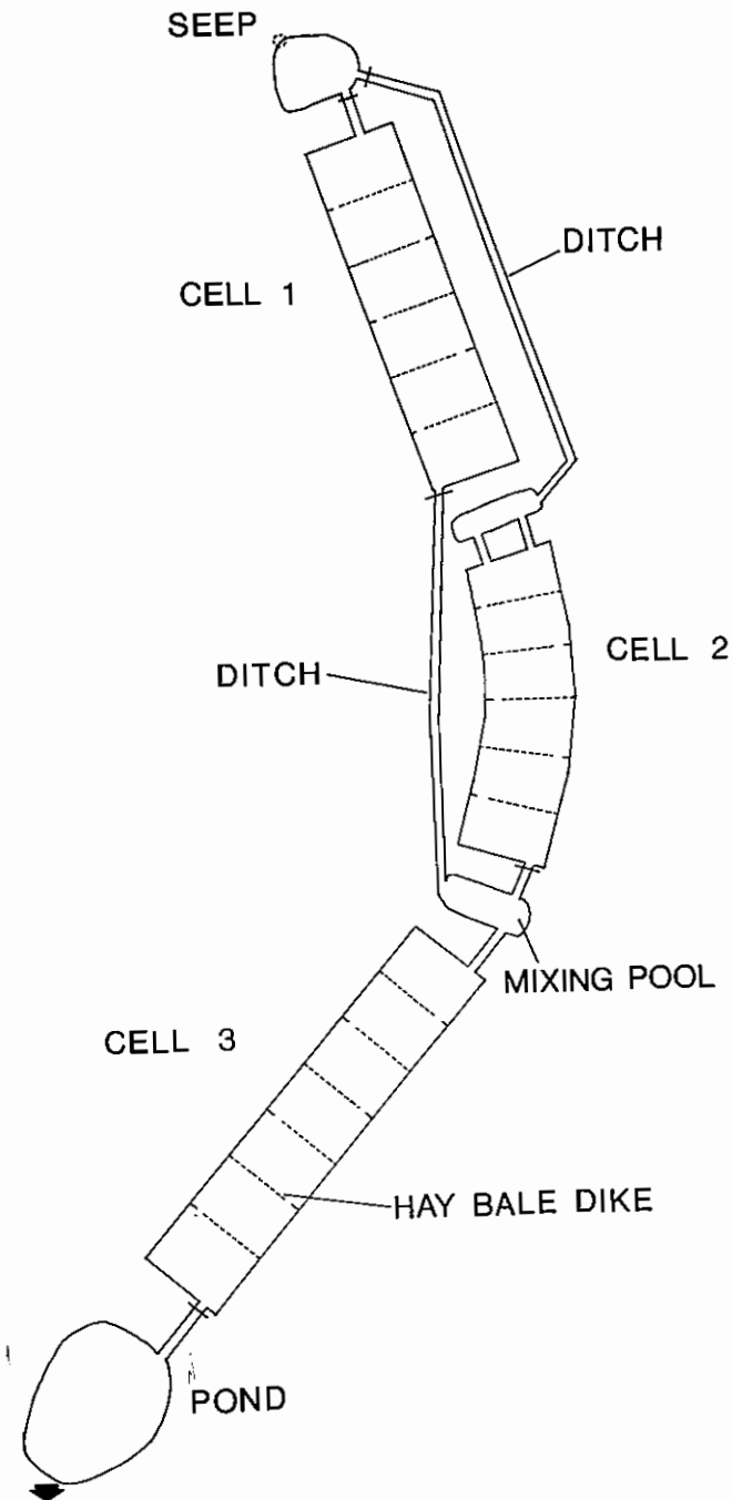
Figure 2.--Diagram of Simco #4 Wetland after site modifications of August 31, 1987. Hay bale dikes were spaced at approximately 35-ft. intervals.
