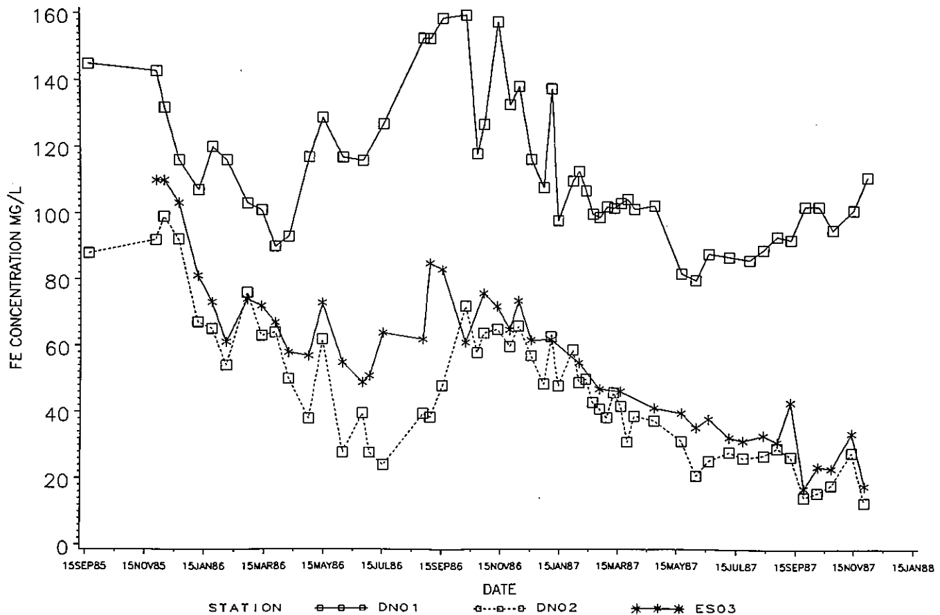
Figure 3.--Total iron concentrations at DNO1 (seep), ES03 (wetland proper outlet), and DNO2 (100-m below wetland).
